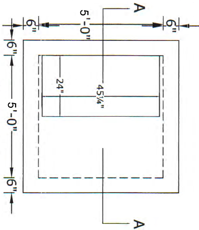
PLAN VIEW
